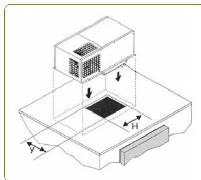
MONOBLOCK TECHO
